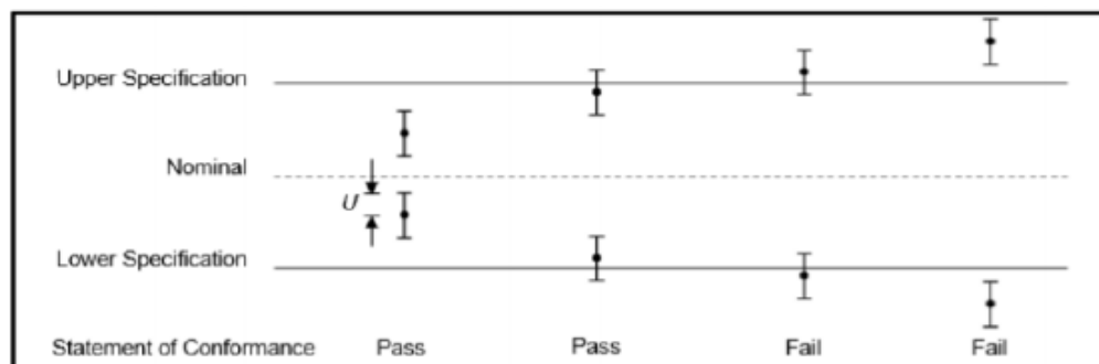
Fig. 1. Graphical representation of a binary statement - Simple Acceptance – acc. to ILAC-G8:09/2019 „Guidelines on decision rules and statements of conformity.”
