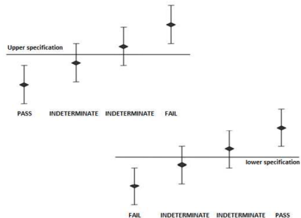
Fig. 3. Graphical representation of a decision rule acc. to ILAC-G8:03/2009 „Guidelines on the Reporting of Compliance with Specification”
